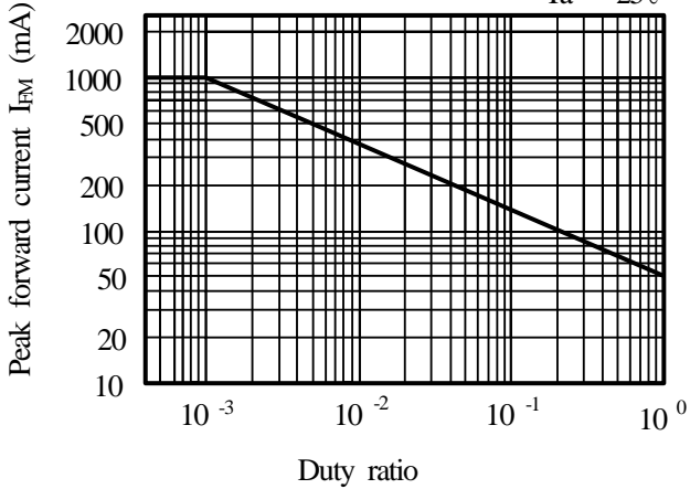
(Fig.7) Forward current vs. duty ratio
